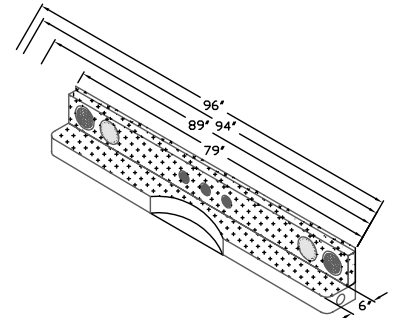
SDB-13 DIAMOND PLATE RECESS STEP BUMPER WITH SEAL BEAM LIGHTS
