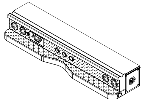
94"x18" Access Door V-Groove Work Deck
