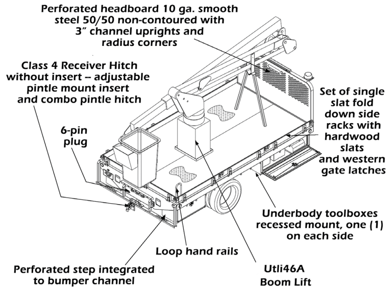
Pictured above is ATA Device on Scelzi 8 x 14 flatbed, WO #108160. Body has PTO and pump for boom lift, back up alarm, basket capacity of 400 lbs, and 540 degree boom rotation with mechanical stop. Meets or exceeds ANSI A92.2-2001 and OSHA requirements
