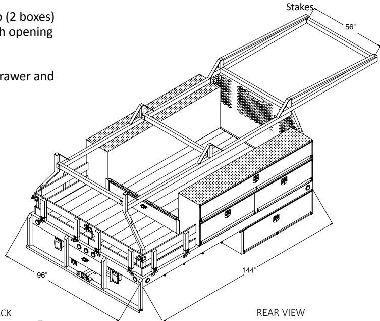
15" Fold Down Side Racks With Aluminum Slats and Stainless Steel Stakes
