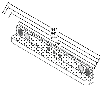
DSB-15 STRAIGHT RAIL DIAMOND PLATE BUMPER WITH SEAL BEAM LIGHTS
