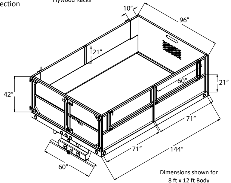
Photo Shows Special Order Removeable Plywood Racks
