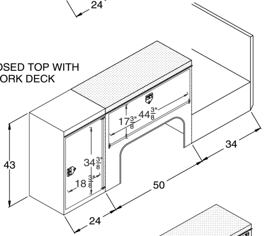
STYLE VO CLOSED TOP WITH 43" TALL COMPARTMENT
