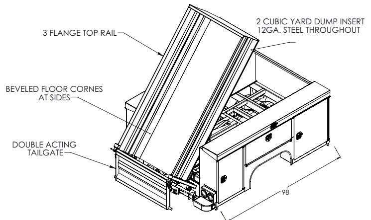
Dimensions for SB-98-79-49-38-VO 2 CUBIC YARD DUMP INSERT
